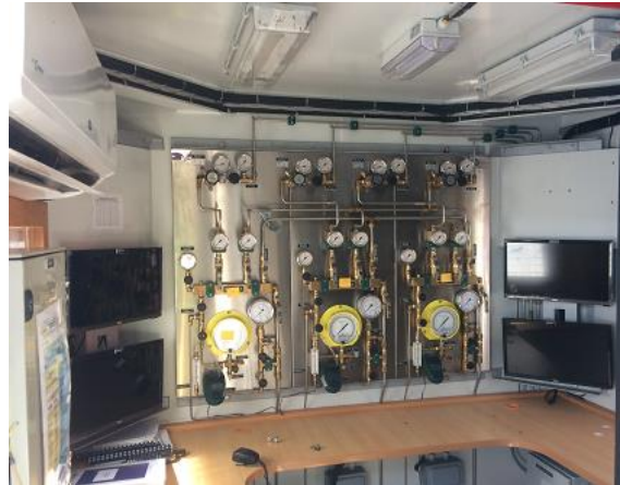
Figure 1: ABS DCON Air Dive Control
